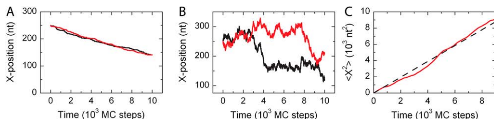
FIGURE 6 Linear motion of a protein. (A) The position of a protein bound to the DNA substrate is followed while allowing unidirectional motion with k_{\text{uni}} = 0.01 (\text{MC step})^{-1} . This yields an approximately linear decrease in time. (B) For a diffusive process with k_{\text{dif}} = 0.01 (\text{MC step})^{-1} , the position of the protein along the DNA substrate displays a random walk. (C) As expected
