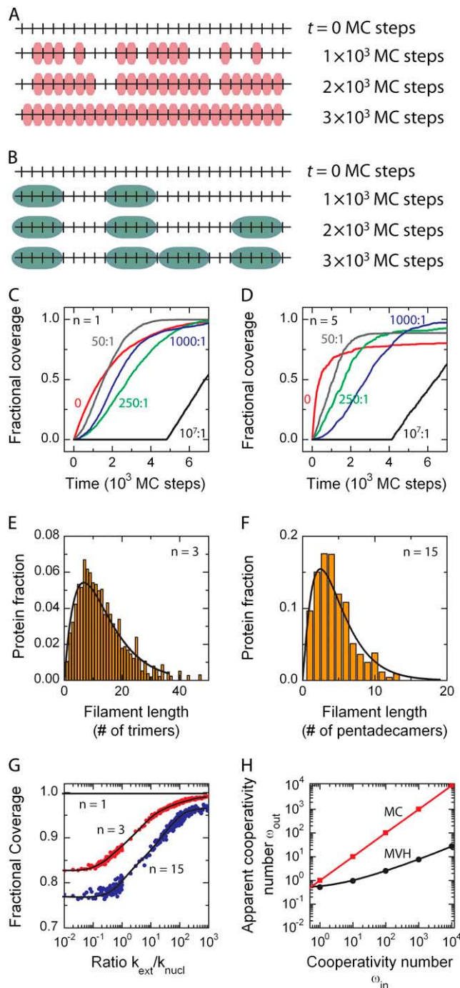
FIGURE 3 Cooperative binding. (A) Snapshots of the DNA occupation by protein at different times during a Monte Carlo simulation for cooperative protein binding. This simulation is carried out for k_{nuc} = 1 \times 10^{-6} site ^{-1} (MC step) ^{-1} , k_{ext} = 5 \times 10^{-5} (MC step) ^{-1} , and a binding size n = 1 . Due to the fast nucleation rate, multiple protein patches are formed along the DNA substrate. Because the protein covers only a single nucleotide or basepair, the final state (bottom panel) is a fully saturated lattice. (B) For a binding size >1 , here n = 5 , a similar intermediate state is observed for equivalent binding rates, but the final state contains gaps since no further proteins can bind. (C) Time-dependent lattice occupancy profiles are obtained from the simulations for different levels of cooperativity. If only random binding (nucleation) occurs along the contour length of the DNA molecule (noncooperative binding; see top left), an exponential lattice occupancy profile
